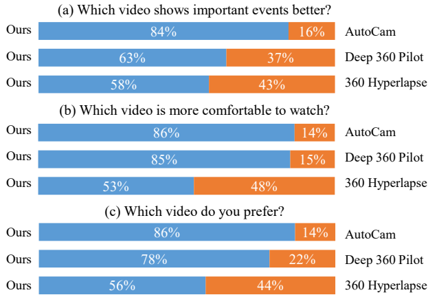
Fig. 16. User study result on comparison with other automatic methods.
