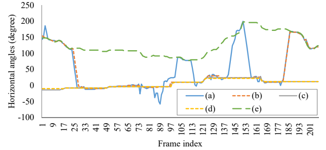
Fig. 6. Different camera paths computed by different methods. (a) Camera path computed by maximizing only saliency. (b)-(d) Camera paths obtained using the conventional smoothness term ((b) \omega_o = 0.01 , (c) \omega_o = 0.05 , (d) \omega_o = 0.1 ). A large \omega_o for the conventional smoothness term makes the path stay at the same position not following salient objects, and a small \omega_o makes the path jump between salient areas. On the other hand, our optical flow-based smoothness term encourages the path to follow salient objects more effectively and stably.
